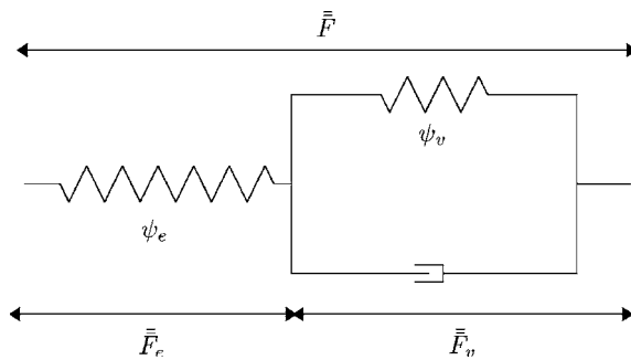
Fig. 2. Poynting–Thomson model.
