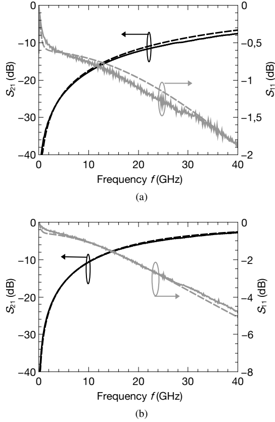
Figure 4. Measured (solid line) and equivalent scheme (dashed line) responses.
