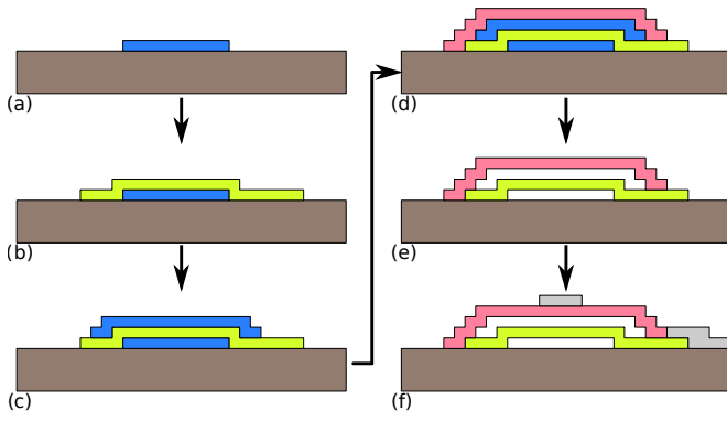
Figure 2. Fabrication steps of the switched capacitor.
