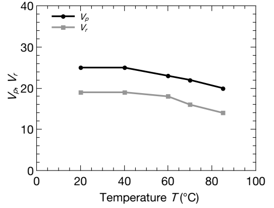
Figure 6. Pull-in voltage V_p and release voltage V_r as a function of temperature.
