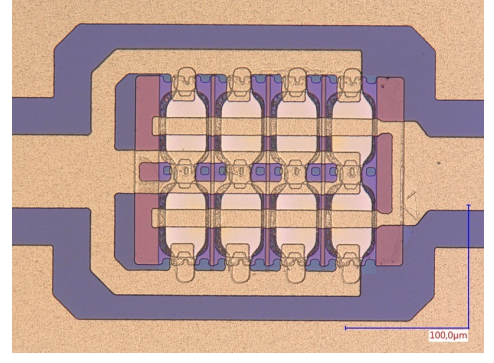
Figure 6. Optical photograph of the capacitor array.
