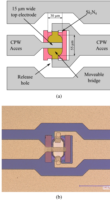
Figure 3. Top view (a) and microphotography (b) of a fabricated switched capacitor.
