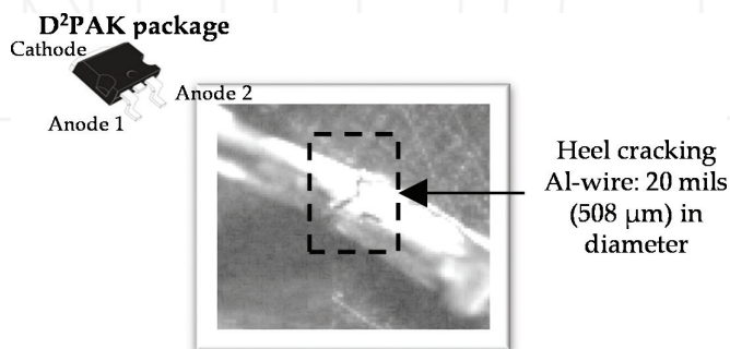
Figure 3. Aluminum wire heel cracking (2 × 20 A, 170-V Schottky diode assembled in a D 2 PAK package).
