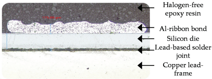
Figure 8. Failure analysis result of a D²PAK package using Al-ribbon bonding after 2000 passive temperature cycles (-65°C/+150°C, two cycles/h).
