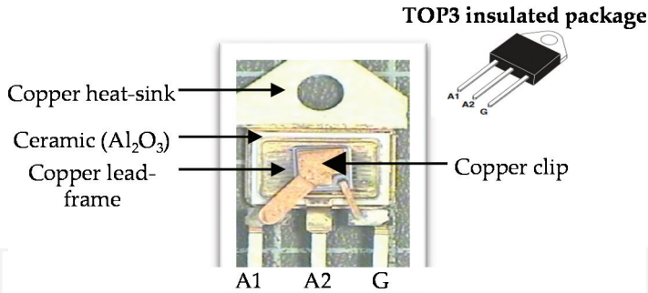
Figure 4. 25 A, 1200-V Triac assembled in a TOP3 insulated package using copper clip bonding.
