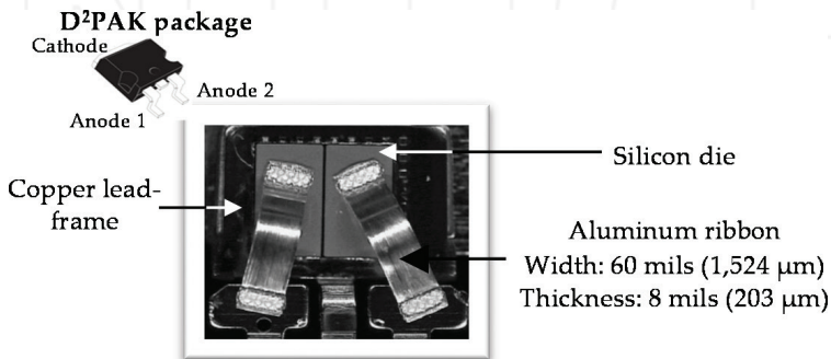
Figure 5. 2 x 20 A, 170-V Schottky diode assembled in a D 2 PAK package using Al-ribbon bonding.
