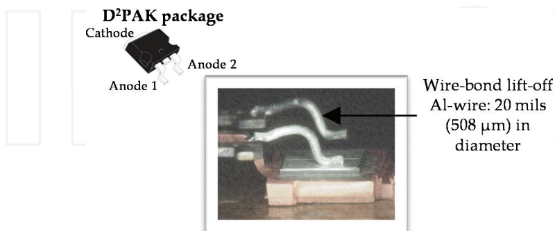
Figure 2. Aluminum wire bond lift-off ( 2 \times 20 A, 170-V Schottky diode assembled in a D 2 PAK package).
