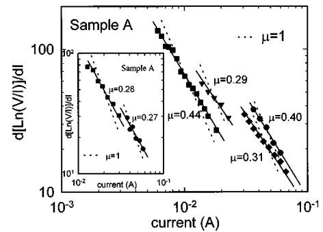
FIG. 7. Log-log plot of d[\ln(V/I)]/dI vs I for B and T fixed in the Bose-glass phase ( \blacksquare f = 0.9 , T = 58.809 K; \blacklozenge f = 0.9 , T = 57.098 K; \blacktriangledown f = 0.04 , T = 74.902 K; \bullet f = 0.04 , T = 72.589 K). The straight lines are regression lines wherefrom we obtain the glassy exponent \mu = 0.33 \pm 0.06 . Inset: \blacksquare f = 0.566 , T = 66.253 K; \bullet f = 0.2 , T = 68.553 K.
