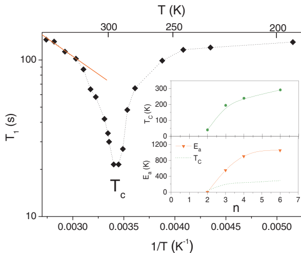
FIG. 1 (color online). Spin-lattice relaxation time as a function of the inverse of temperature for p -6P. The straight line fits the activated behavior. The inset displays the variations of the critical temperature T_c (upper panel) and the activation energy E_a (lower panel) compared to T_c (dotted line) for the p - n P as a function of the number of phenyl rings ( n ).
