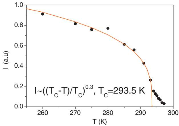
FIG. 2 (color online). Temperature dependence of averaged x-ray intensity of the superstructure reflections (1.5,1.5,1) and (-1.5, 1.5, -1) measured on a single crystal of p-6P .
