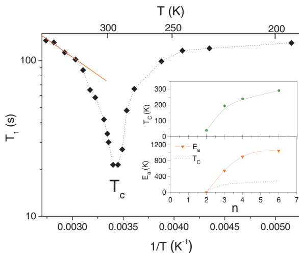
FIG. 1 (color online). Spin-lattice relaxation time as a function of the inverse of temperature for p -6 P . The straight line fits the activated behavior. The inset displays the variations of the critical temperature T_c (upper panel) and the activation energy E_a (lower panel) compared to T_c (dotted line) for the p - n P as a function of the number of phenyl rings ( n ).
