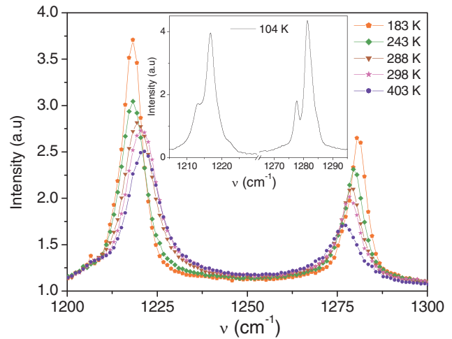
FIG. 3 (color online). Raman spectra at various temperatures obtained on single crystals of p-6P . The inset exhibits the more complex structure of these modes at low temperature.
