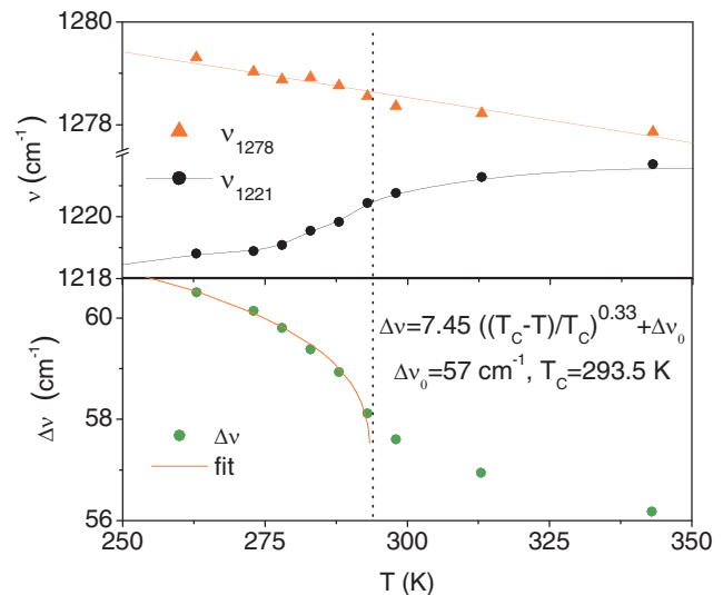
FIG. 4 (color online). Variation of the frequencies of the two main Raman modes \nu_{1278} and \nu_{1221} as a function of temperature (upper panel). The lower panel displays the temperature dependence of the difference \Delta\nu = \nu_{1278} - \nu_{1221} , where the subscripts indicate the high temperature frequencies.
