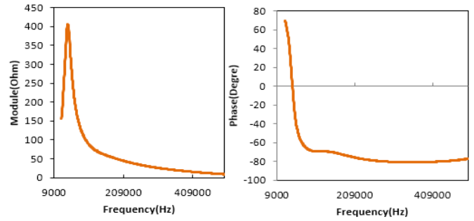
Fig. 12. Z_{\text{installation}} without loads
