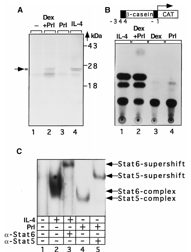
FIG. 1. Lactogenic-hormone induction of Stat5 and IL-4 induction of Stat6 activate \beta -casein gene transcription in mammary epithelial cells. (A) HC11 mammary epithelial cells were treated with no hormones (-; lane 1), dexamethasone, and prolactin (Dex + Prl) (lane 2), prolactin (lane 3), or IL-4 (lane 4). Whole-cell protein extracts were prepared, separated by gel electrophoresis, and analyzed by Western blotting with a mouse \beta -casein-specific antiserum. The arrow and horizontal lines indicate the positions of differently phosphorylated forms of \beta -casein. (B) HC11 cells stably transfected with a \beta -casein promoter-CAT construct were treated with IL-4 (lane 1), dexamethasone and prolactin (lane 2), dexamethasone (lane 3), or prolactin (lane 4). Four independent experiments were carried out, with similar results. (C) Bandshift assays of Stat6 activated (+) by IL-4 (lanes 2 and 3) and Stat5 activated by prolactin (lanes 4 and 5). Whole-cell extracts were prepared and introduced in bandshift assays. The proximal \beta -casein promoter Stat binding site served as the probe. Supershifts were carried out with (+) a polyclonal antiserum directed against Stat6 (633 to 837) ( \alpha -Stat6; lane 3) or Stat5 ( \alpha -Stat5; lane 5).
