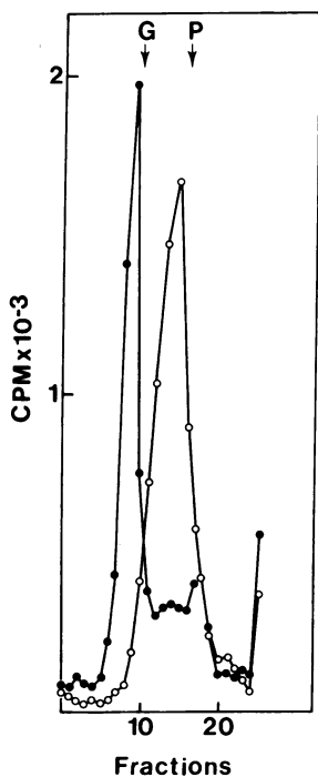
FIG. 1. Glycerol gradient centrifugation. Samples containing 8-9S [ ^3\text{H} ]ICI-ER complexes were analyzed by sedimentation in a 10-35% glycerol gradient with low salt (●) or high salt (0.4 M KCl) (○). The samples were centrifuged in a Beckman SW60 rotor at 220,000 \times g for 15 hr. Arrows indicate the sedimentation of internal standards: G, glucose oxidase (7.9 S); P, peroxidase (3.6 S).
