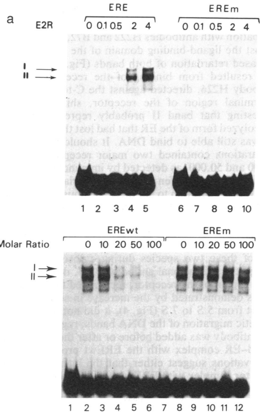
FIG. 2. Sequence-specific binding of ER to the ERE. (a) Binding reaction mixtures contained 0.05 ng of EREwt (lanes 1-5) or EREm (lanes 6-10) probe and 0.1, 0.5, 2, or 4 ng of receptor bound to \text{E}_2 (E2R). (b) Unlabeled competitor oligonucleotides were included in the binding reaction mixture prior to addition of \text{E}_2 -ER (4 ng). The molar ratio of competitor over the labeled probe (EREwt, 0.05 ng) is indicated above each lane. Protein-DNA complexes were separated from protein-free DNA by polyacrylamide gel electrophoresis and visualized by autoradiography.
