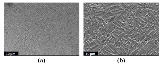
Fig. 4. SEM observations of the LMD parts (a) in the as build state and (b) after the HIP treatment (section parallel to XY plane).
