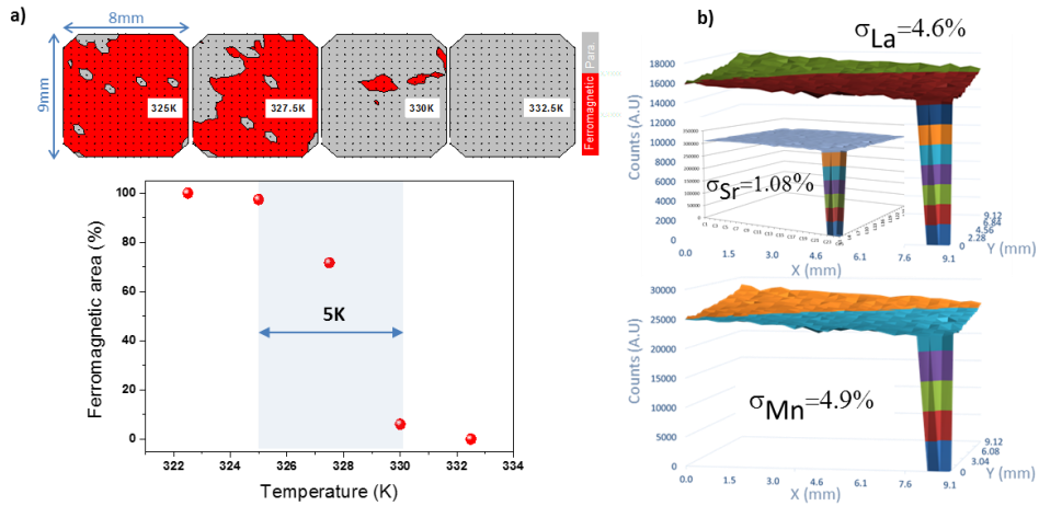
Figure 6. (a) Magnetic state maps of LSMO 20 uc film at various temperature (top) and T_c distribution at the sample surface (bottom). (b) WDS signal for La, Sr and Mn over 9 \times 9 mm 2 of the same sample.
