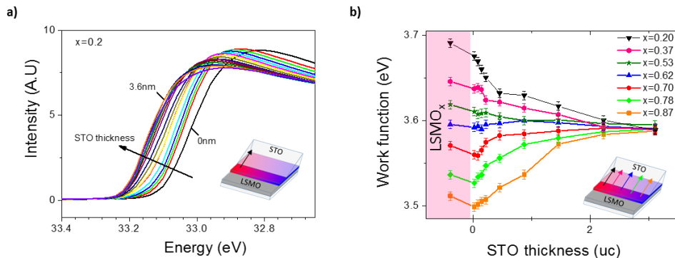
Figure 11. (a) HeII UPS threshold for various t_{STO} at x=0.2 U_{bias} = 4V . (b) Corresponding extracted W_F versus t_{STO} for various Sr content x
