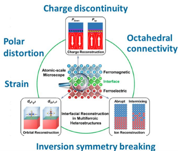
Figure 5. Schematic of competing interactions and phenomenon at perovskite \text{ABO}_3 interfaces. From [26] with permission.
