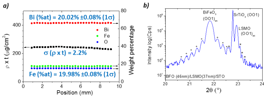
Figure 2. (a) Evolutions of density \times thickness product ( \rho\cdot t ) and weight percentages of Bi, Fe and O as a function of the position and (b) X-Ray diffraction pattern of BFO/LSMO/STO heterostructure
