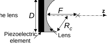
Figure 3 : Lens-focused transducer.
