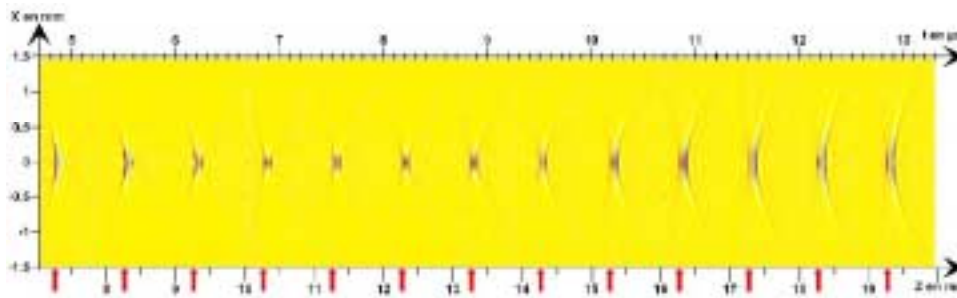
Figure 24 : Spatio-temporal evolution of acoustic beam (20 MHz transducer) between z=7 and 19\text{mm} ( 1\text{mm} step).
