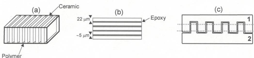
Figure 10 : (a) Schematic representation of a 2-2 piezo-composite sample. (b) Schematic cross-section of a high frequency 2-2 piezo-composites used. (c) Schematic representation of Interdigital Pair Bonding process.
