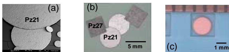
Figure 7 : Tape-casted self supported disk photographs. (a) (b) from Ferroperm piezoceramics (Denmark), (c) from Laboratoire de Céramique (EPFL, Switzerland).
