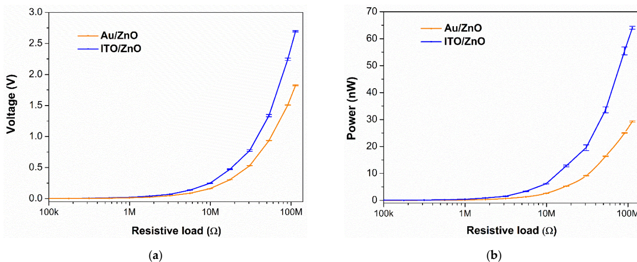
Figure 9. RMS output voltage (a) and average power (b) generated by PENGs with different seed layer structures. Measured RMS voltage and average power for a load resistance ranging from 100 kΩ to 100 MΩ, when applying an alternative mechanical excitation with a magnitude of 3 N at a frequency of 5 Hz.
