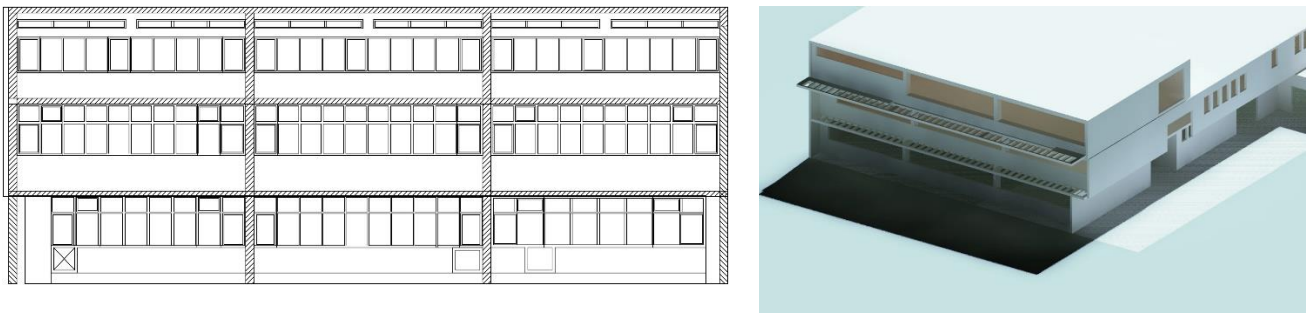
Figure 8. Two-dimensional drawing of the East façade and view of the three-dimensional model.
