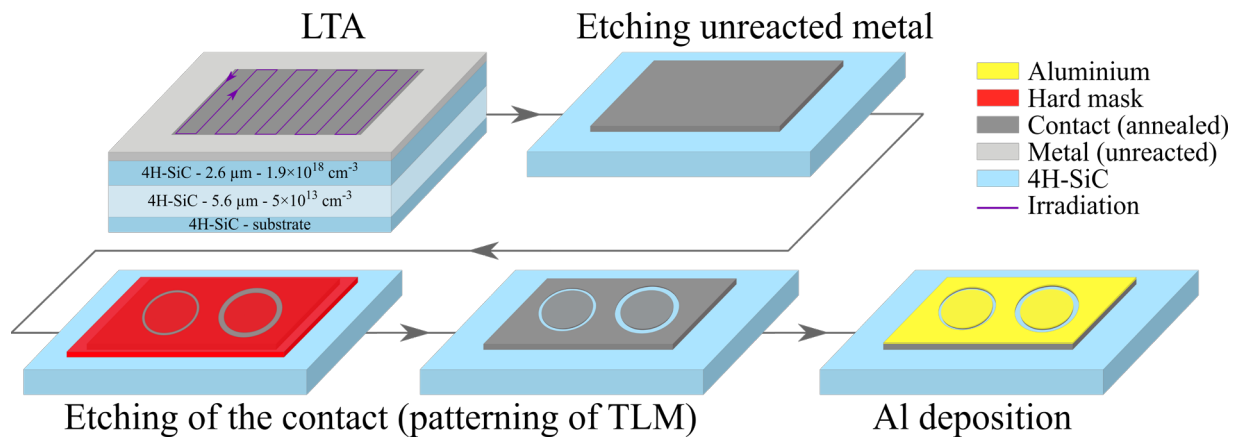
Fig. 1: Schematic representation of the fabrication process used to define the TLM structures.
