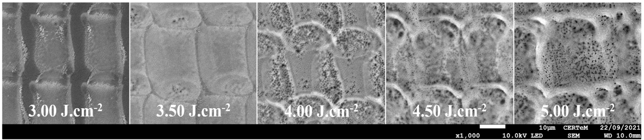
Fig. 4: SEM images of Ti annealed between 3.0 and 5.0 \text{J.cm}^{-2} at 800 \text{ mm.s}^{-1} .
