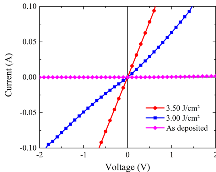
Fig. 3: I-V characteristics for a tests structures made of Ti/4H-SiC contact annealed at 185 \text{ mm.s}^{-1} .
