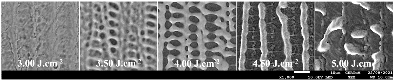
Fig. 2: SEM images of Ti annealed between 3.0 and 5.0 \text{J.cm}^{-2} at 185 \text{ mm.s}^{-1} .
