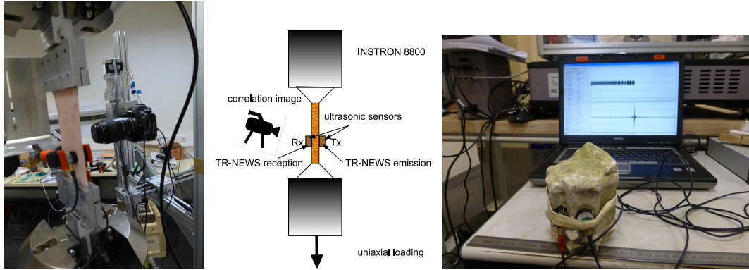
Figure 2: TR-NEWS experimental set-up for acousto-mechanical imaging of the porcine skin aging (a,b) and for the aging characterization of Tuffeau limestones
